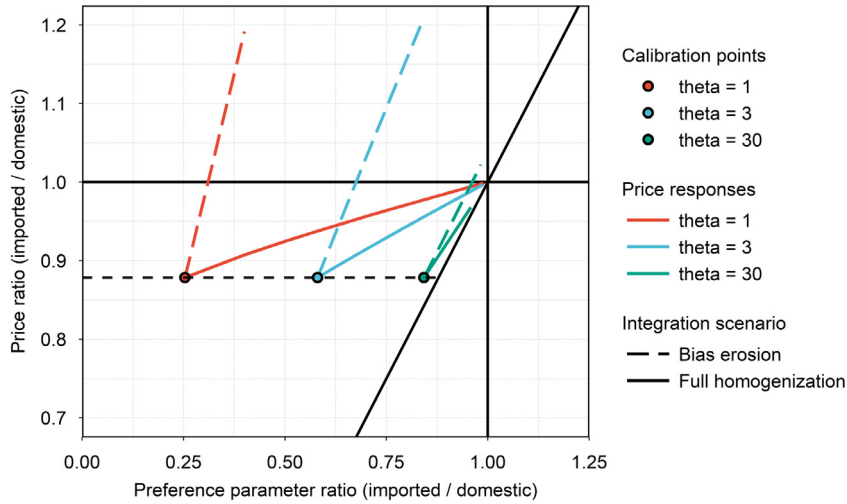
Fig. 2. Price responses to comparative static preference shocks across market integration scenarios. The calibrations points show the relationship between initial price ratio and calibrated preference parameter ratio given an initial \theta_0 . Note that the diagonal black is 45-degree line. Lines (distinguished by integration scenarios) are simulated by implementing comparative static shocks of \delta_n (bias erosion scenario) or \theta_n (full homogenization scenario) in the theoretical model (Section 2.1). The theoretical model is calibrated to 1995 Asian soybeans data for different initial theta ( \theta_0 equals 1, 3, or 30) with other parameters of \eta^D = -0.5 , \xi_d^S = \xi_m^S = 0.5 , and p_o = e = 0 .
