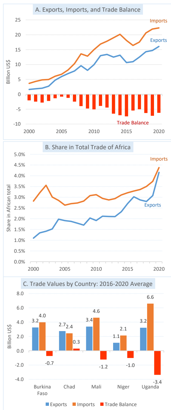
Figure 3: Trade Performance of the Landlocked OIC Countries in Africa
