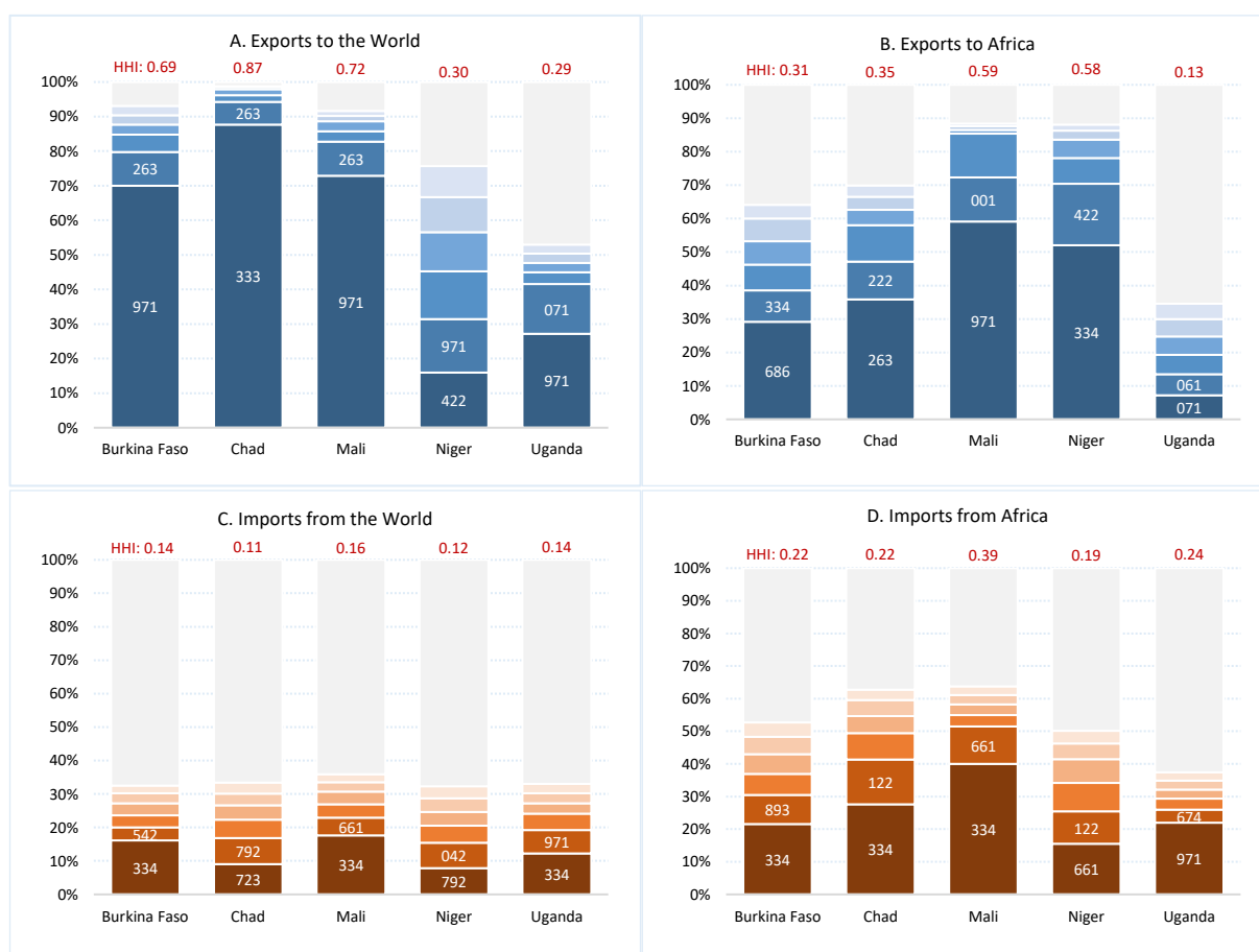
Figure 5: Major Products Exported/Imported by Landlocked OIC Countries in Africa (by SITC 3-digit commodity group*, 2016-2020 average, % of total)
