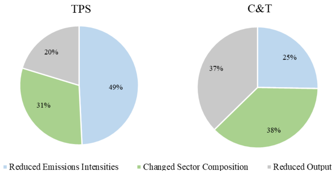
Figure 6. Sources of Emissions Reductions Under the TPS and C&T, 2020-2035
