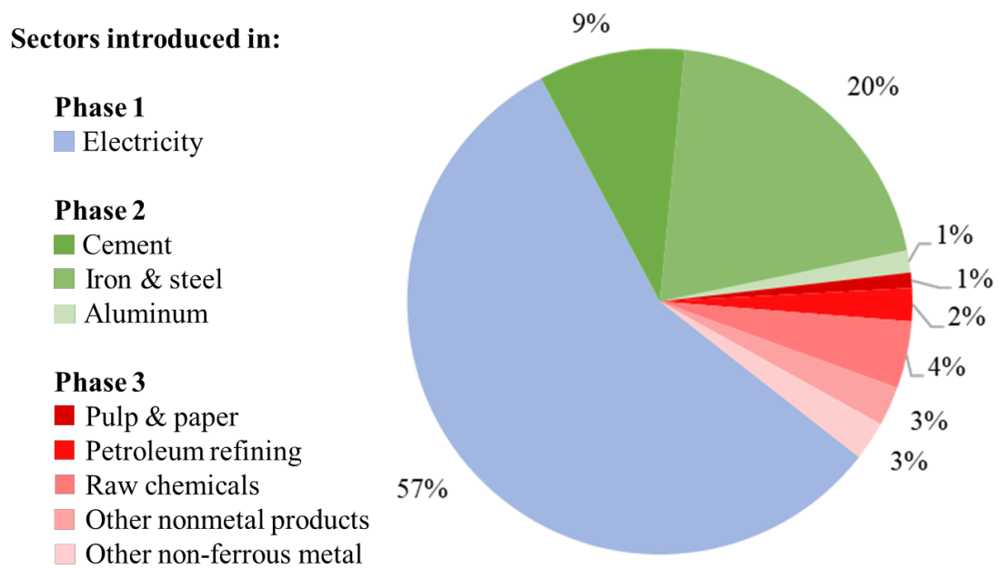
Figure 3. Covered-Sectors' Cumulative Emissions Reductions Over the Interval 2020-2035
