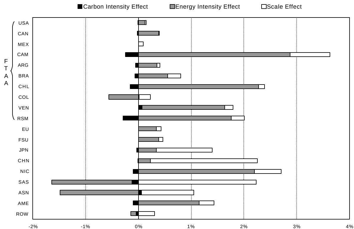
Figure 7: Decomposition of Percentage Change in CO 2 Emissions Following Worldwide Trade Liberalization
