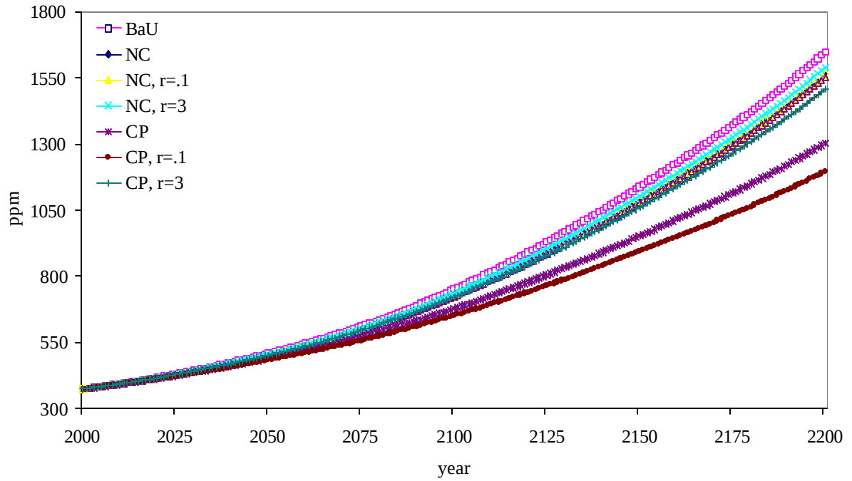
Figure 5. The atmospheric concentration of carbon dioxide according to the business as usual (no control scenario), three non-cooperative optimal emission control scenarios with alternative values for the pure rate of time preference, and, three cooperative optimal emission control scenarios with alternative values for the pure rate of time preference.
