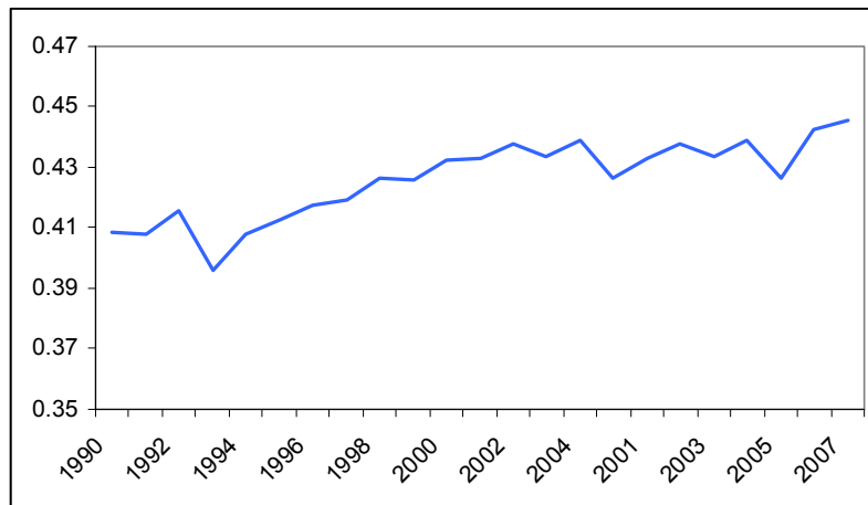
Graph 1: Gini Index
