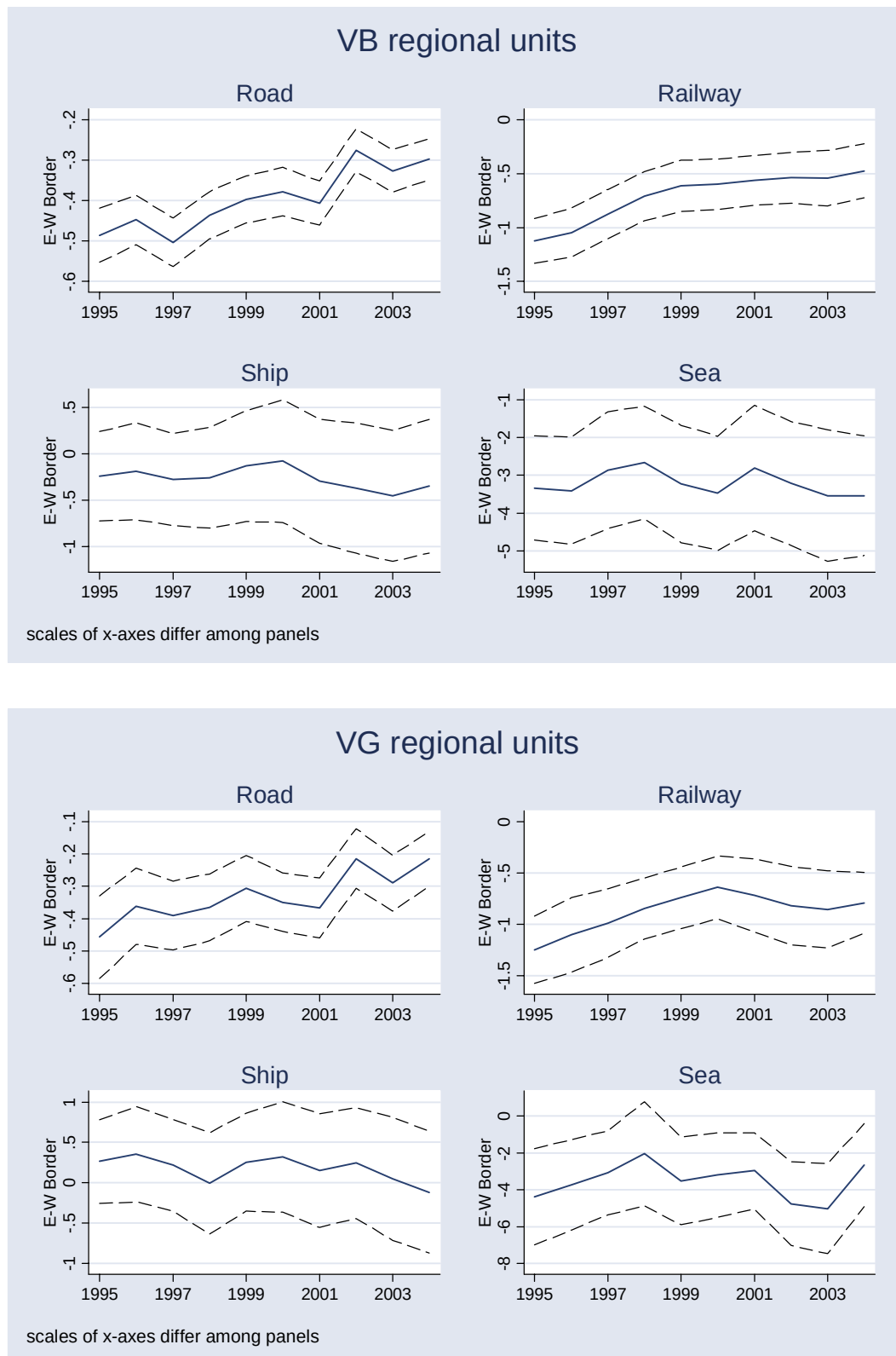
Figure 3: Estimation Results by Mode of Transportation
