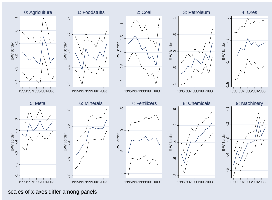
Figure 4: Estimation Results by 1-Digit Industry
