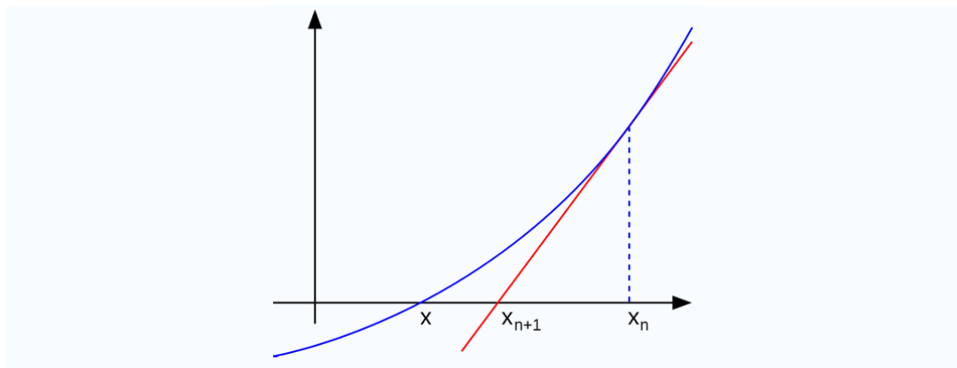
Figure 3 Newton's method
