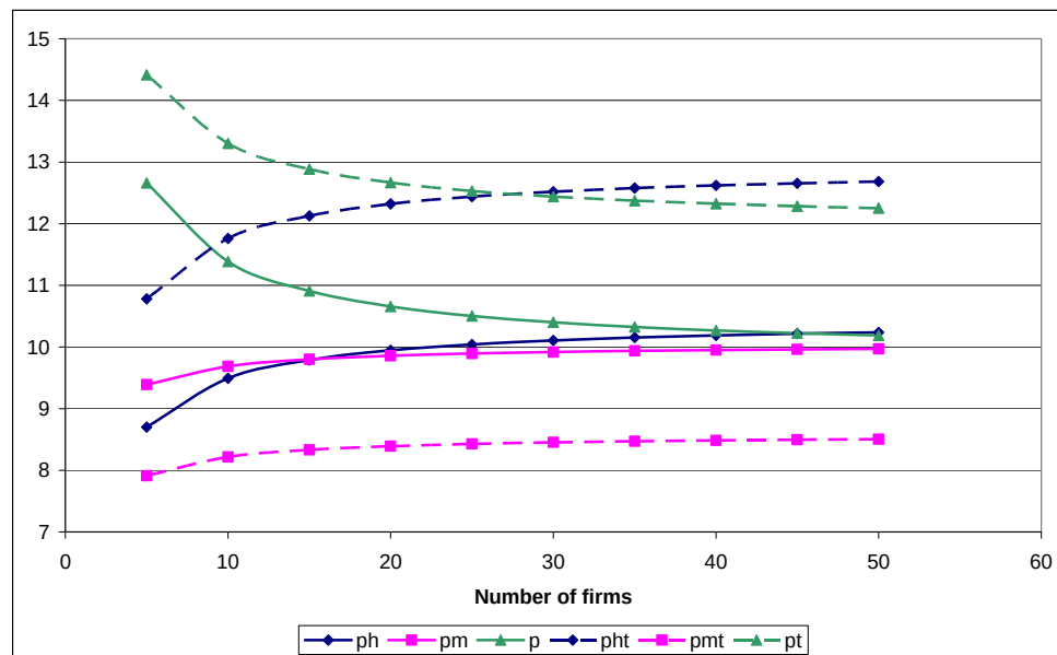
Figure 3: Means of Prices as a Function of n with a 25% Tariff
