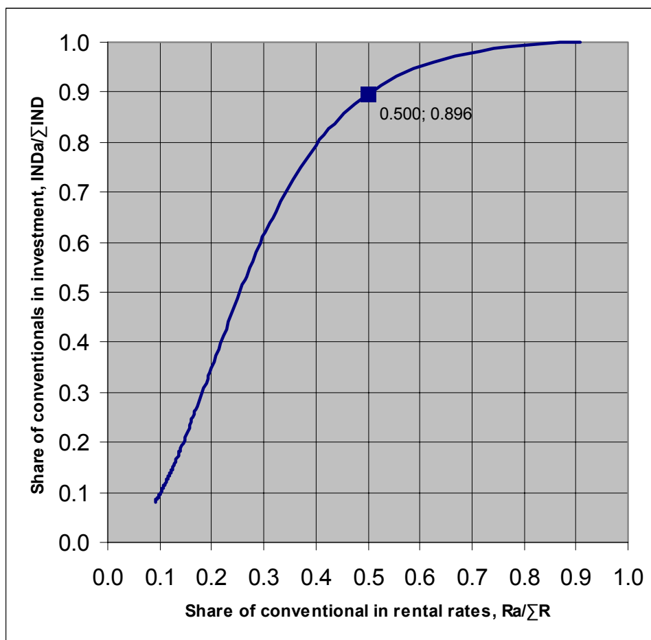
Figure 1: Standard investment function (INVFN=1)
