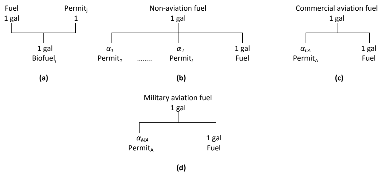
Figure 5. Implementation of RFS2 mandates and the aviation biofuel goal in the EPPA-A model (a) Production of permits ( j = corn ethanol, other advanced, cellulosic, and renewable jet fuel), (b) Blending of permits into non-aviation fuel, (c) Blending of permits into commercial aviation fuel, and (d) blending of permits into military aviation fuel.
