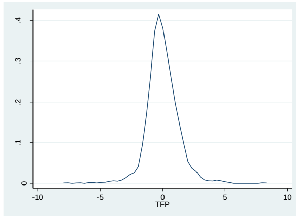
Figure 4: Kernel Density Estimate for TFP
