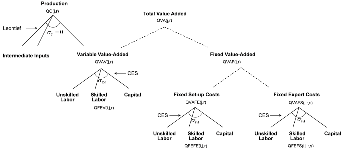
Figure 1. Production Tree and Value-Added in the Monopolistically Competitive Sector in GTAP-HET
