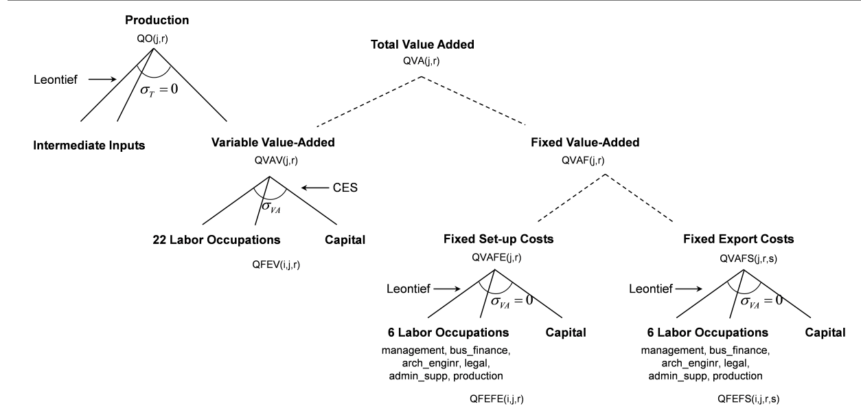
Figure 4. Modified Production Tree and Value-Added with Changed U.S. Labor Categories
