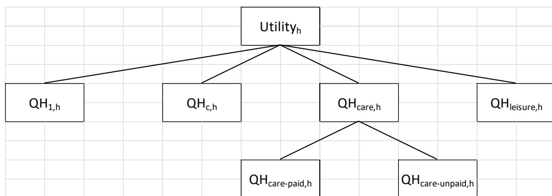
Figure 2.1: utility function
