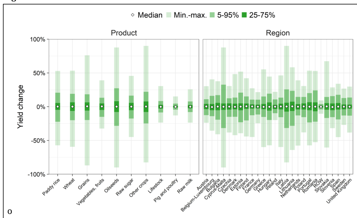
Figure 2: Yield shocks
