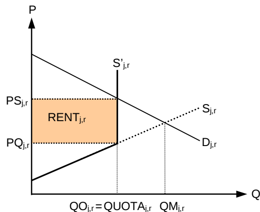
Figure 1: Output quota of sector j in region r
