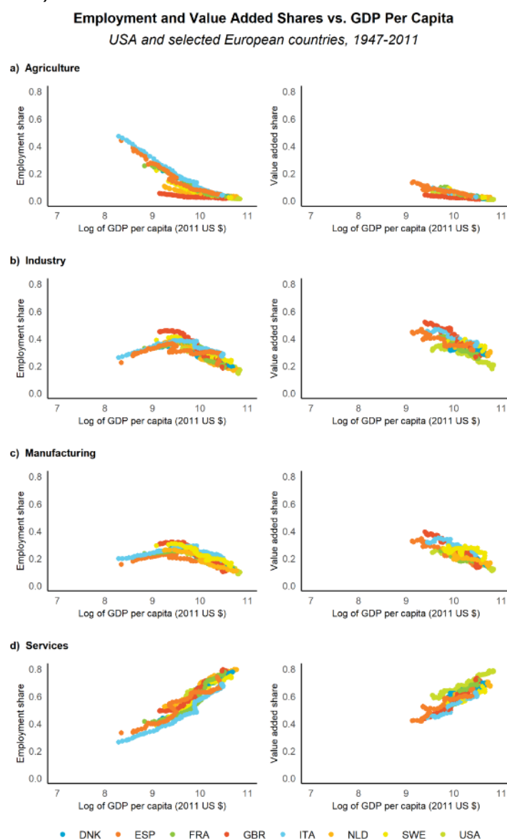
Figure 1: Sectoral Shares of Employment and Nominal Value Added – Selected European Countries and the USA, 1947–2011.
